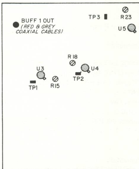
Figure 4-3. Test points and adjustments for filter alignment.
