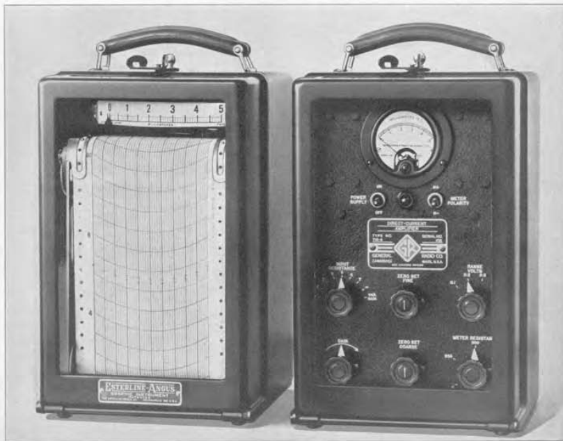
FIGURE 1. TYPE 715-A Direct-Current Amplifier and Esterline-Angus 5-milliamperer recorder. The amplifier can be obtained in a case to match the recorder as shown here, or in a walnut cabinet as shown on page 3. A relay-rack mounting to hold both the amplifier and the recorder is also available.
