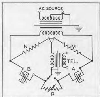
FIGURE 2. Wiring diagram for TYPE 216 Capacity Bridge
